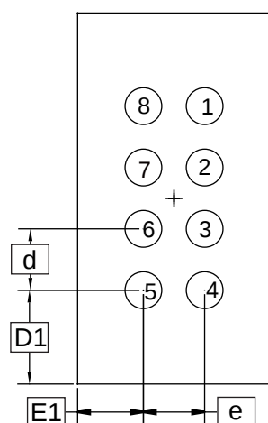
Bottom View
