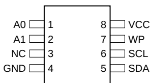
8-lead SOIC
